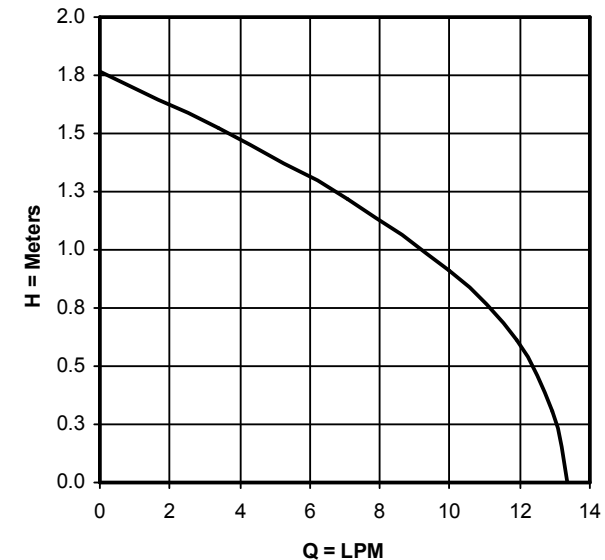
1 230V 50Hz
