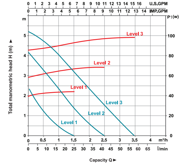
LRP25-60/130 — Q-H — Q-P
